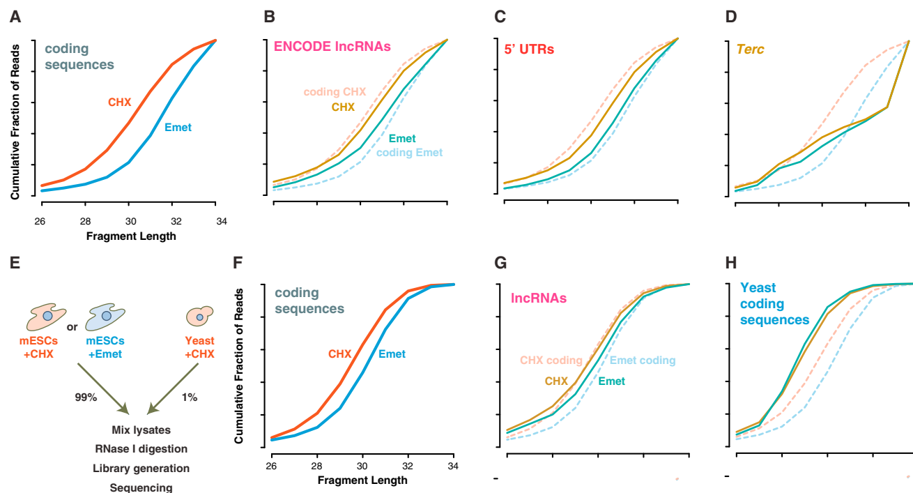
Figure 2. Elongation Inhibitors Shift Ribosome Footprint Sizes
