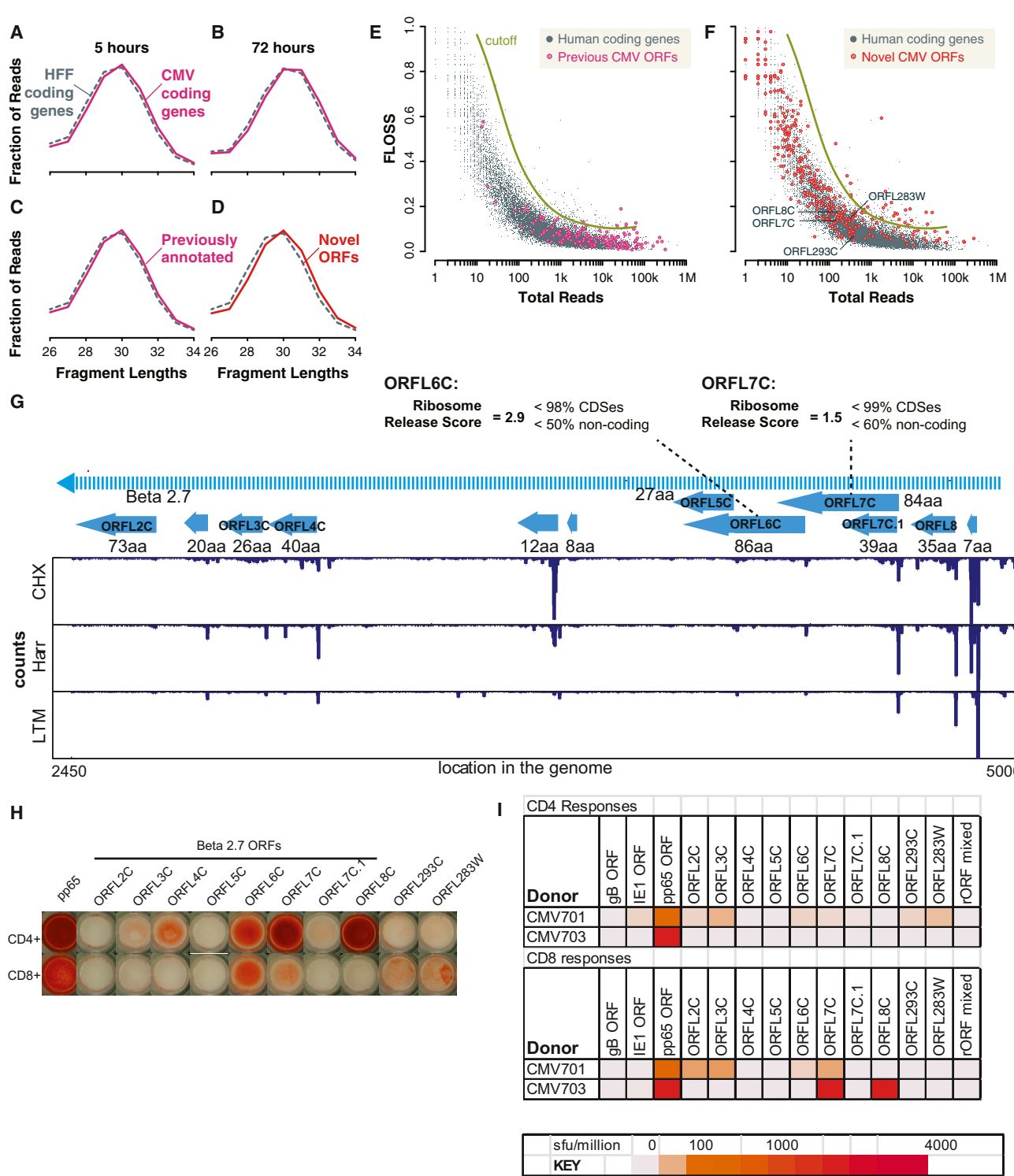
Figure 6. Novel Human Cytomegalovirus Reading Frames Based on True Ribosome Footprints Lead to Antigens in Humans (A–D) Distribution of fragment lengths mapping to human nuclear CDSs compared to all annotated CMV-coding sequences after (A) 5 hr or (B) 72 hr of infection and of specifically the (C) previously annotated and (D) novel CMV-coding sequences after 5 hr of infection. (E and F) Fragment length analysis of human coding sequences compared to (E) previously annotated CMV reading frames and (F) novel CMV annotations. (G) Ribosome footprint organization on beta 2.7 transcript (Stern-Ginossar et al., 2012). (H) ELISPOT assay of human donor T cell responses to novel CMV reading frames along with controls. (I) Quantitation of ELISPOT data.
